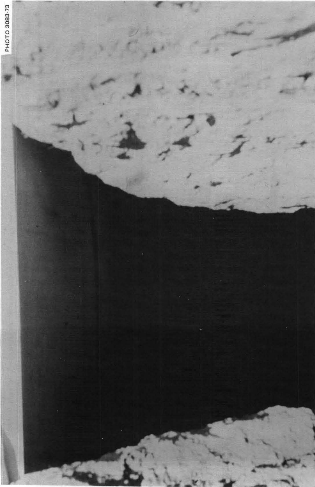
Fig. 3.4. View of interior doors after the successive loadings shown by the preceding photos. The center doors had been bowed downward a total of about 1\frac{1}{2} in.
